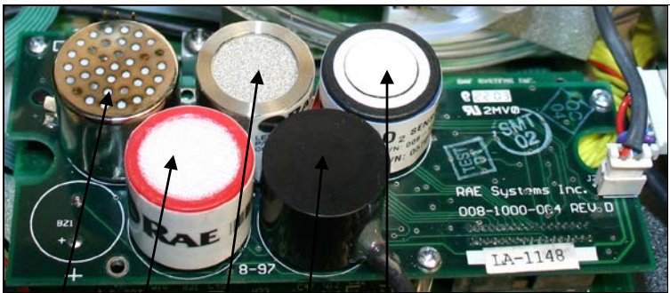
Figure 6-2 Gas Plate of AreaRAE
